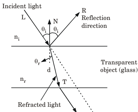
Fig. 5.14.1. Refraction light.
